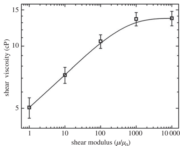
Figure 2. Functional dependence of shear viscosity of sickle RBC suspensions on the normalized shear modulus obtained from DPD simulations.
