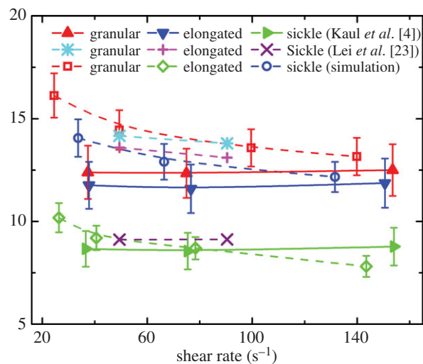
Figure 1. (a) Shear viscosity of healthy blood at Hct = 45% and (b) sickle RBC suspensions at Hct = 40% with different cell morphology. For comparison, the experimental measured shear viscosity of whole blood in health at Hct = 45% by Chien et al. [34] and in SCA at Hct = 40% by Kaul et al. [4], and previous computational simulations of sickle RBC suspensions at Hct = 40% by Lei et al. [23] are shown in these figures. The dashed line in panel (a) represents the fitted curve to the simulation result by \eta = be^{-a/\dot{\gamma}^{b.5}} + c , where \dot{\gamma} is the shear rate; a , b and c are 6.6 \times 10^{-3} , -2374.7 and 2378.0 , respectively. (Online version in colour.)
