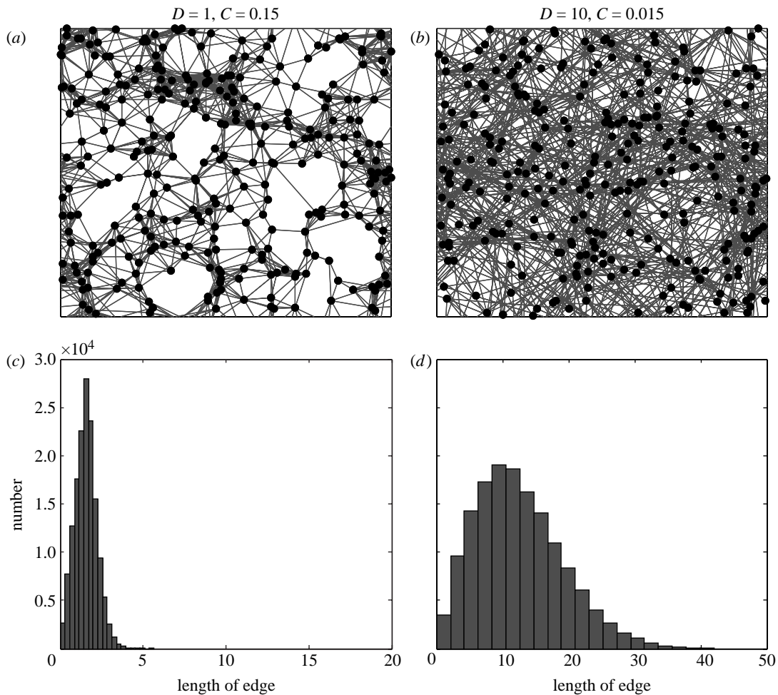
Figure 1. Graphs with two different D values. (a,c) D=1 . (b,d) D=10 . Clustering coefficients ( C ) are calculated using the formula in appendix A. While the degree distribution and average number of contacts for each of these graphs are similar, the average length of each of these connections is much higher on the D=10 graph (note that different length-scales are used for c and d). To allow better visualization of the networks, these graphs have 300 individuals and n (average degree) = 8; graphs used for the simulations have 100 000 individuals and n=15 .
