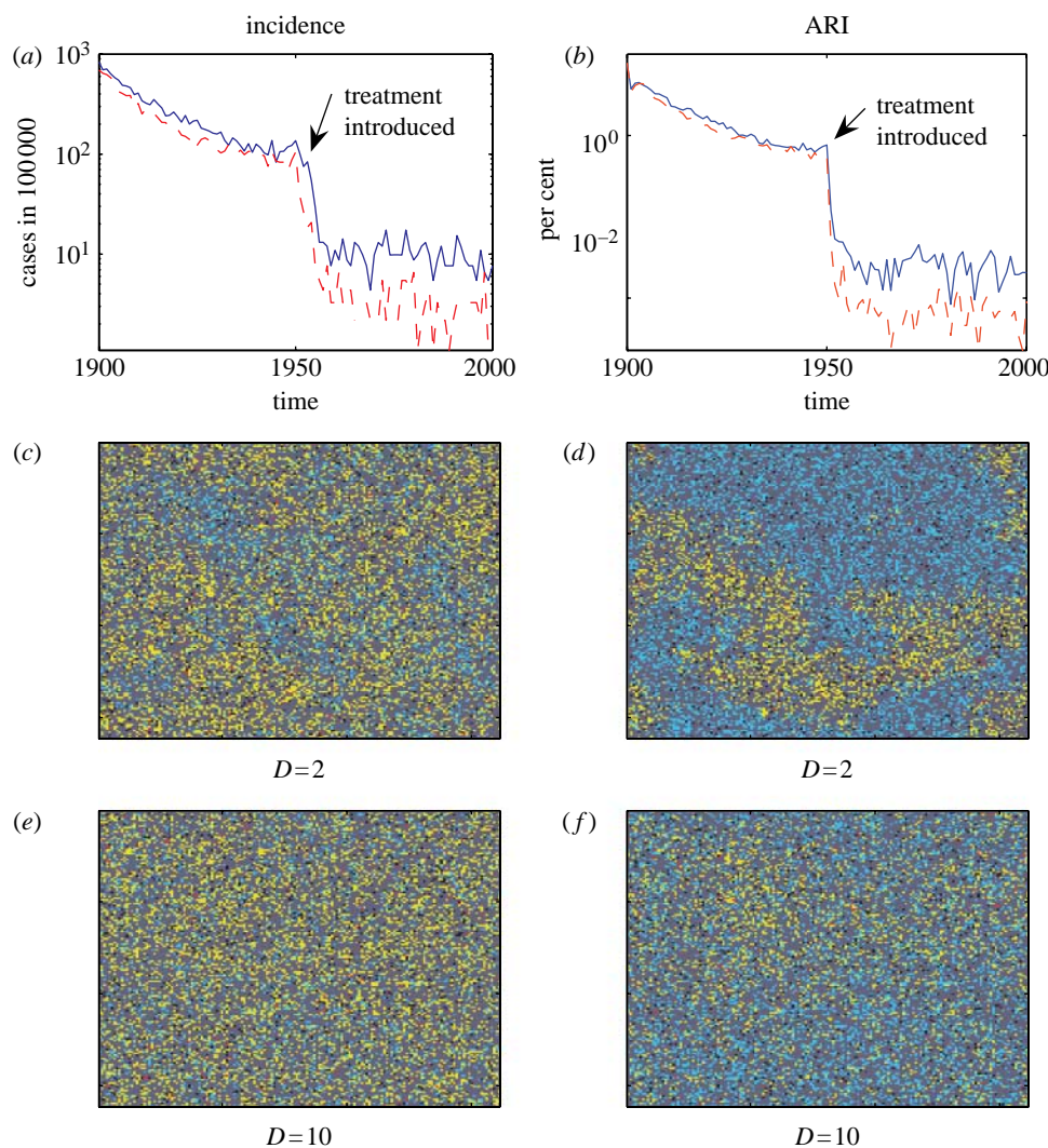
Figure 3. Simulations. (a) TB incidence and (b) ARI on graphs with D=2 (dashed orange) and D=10 (solid blue) with 100 000 individuals and parameter values as listed in table 1. Snapshots showing 10 000 individuals during epidemics at (c, e) high and (d, f) low incidence on graphs of (c, d) D=2 and (e, f) D=10 . Grey pixels are unoccupied spaces, blue pixels represent individuals who are susceptible to infection and yellow pixels represent individuals with latent infection. Even at incidence levels considered high for TB epidemics, infectious individuals (red) are not present in large enough numbers to be seen easily at this resolution and edges are not shown in this representation as they were in the much smaller network depicted in figure 1 a, b . Clustering of those with latent infection is evident in the more local graph at low levels of incidence (d), but not easily detected at higher incidence (c) or on the more global graph at any time in the epidemic (e, f).
