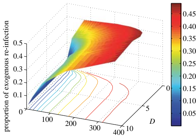
annual incidence of TB (cases in 100000)
