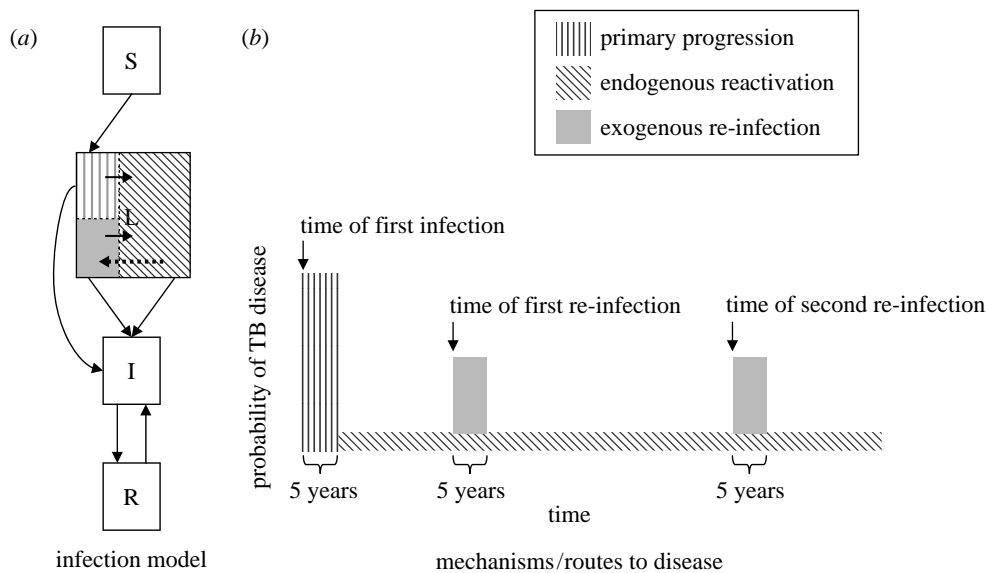
Figure 2. Disease model transitions. (a) Infection model. Individuals are born into the susceptible state (S); if infected they move into a state of latency (L) from which they suffer primary progression to disease (vertical grey bars) for the first 5 years after infection, endogenous re-activation (diagonal black bars) if they progress to disease more than 5 years after an infection (or re-infection) event or exogenous re-infection (dark grey) if they progress to disease within 5 years after a re-infection event. Individuals in the diseased state (I) are infectious until they are either cured by drugs and move to the recovered state (R) (in our simulations this happens only after drugs become available in 1950), they self-recover and return to latency (arrows not shown), or they die. (b) Routes to disease. Progression for a hypothetical individual who is infected three times over the course of his life. The height of the bars represents the probability of progression to disease (by each route) as a function of time.
