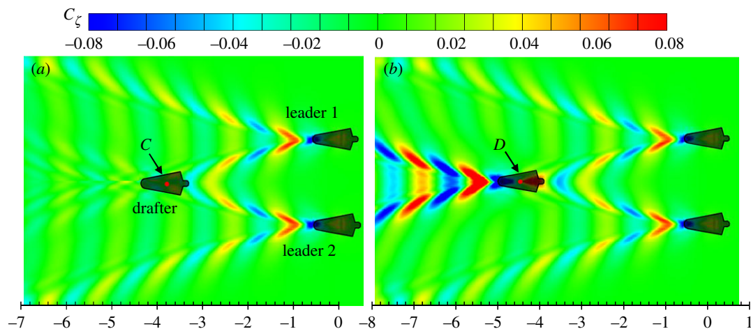
Figure 12. Wave patterns generated by three swimmers in a V-shape configuration at d_t = 2.0 m and U = 2.0 m s -1 . (a) Drafter is located at position C; (b) drafter is located at position D. The x -axis is the non-dimensional longitudinal distance d_1/L . (Online version in colour.)
