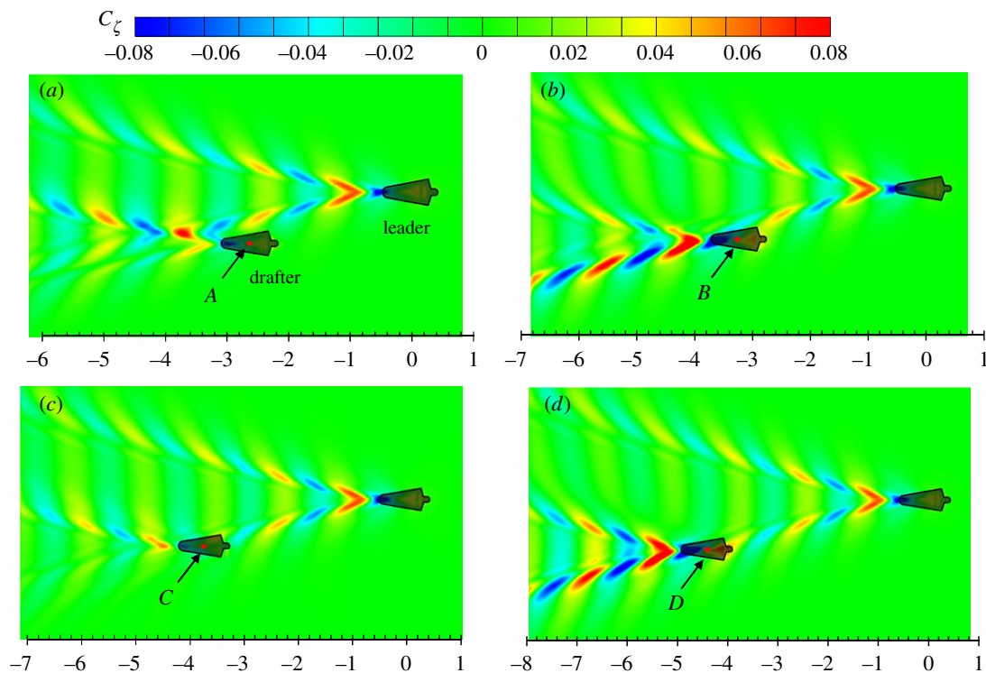
Figure 10. Wave patterns generated by two swimmers at d_t = 2.0 m and U = 2.0 m s^{-1} . The x -axis is the non-dimensional longitudinal distance d_i/L . Four typical positions are selected, namely A , B , C and D , which represent the peak values in corresponding boxed regions in figure 9. (Online version in colour.)
