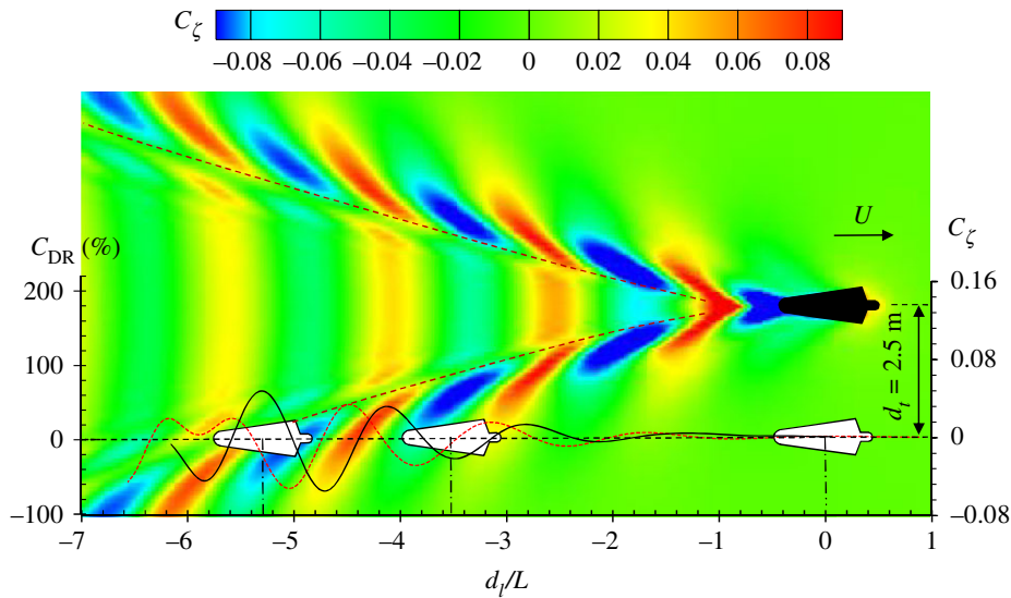
Figure 8. Wave drag reduction coefficient (black solid curve) of a drafter when he/she swims alongside a leader at U = 2.0 \text{ m s}^{-1} . The colour contour indicates the wave pattern generated by the leader. The red dash curve is the wave profile at the moving path of the drafter. (Online version in colour.)
