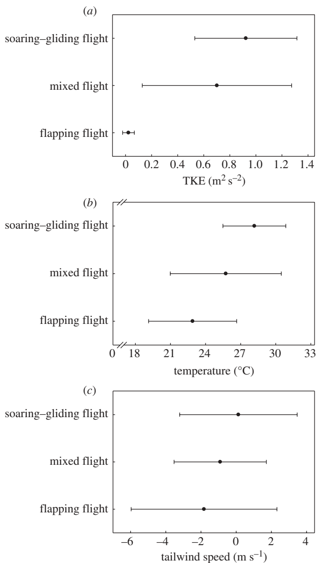
Figure 2. The relationships between meteorological variables simulated at 500 m above-ground and bird flight mode. (a) TKE, (b) temperature and (c) tailwind. For statistical details see table 1.
