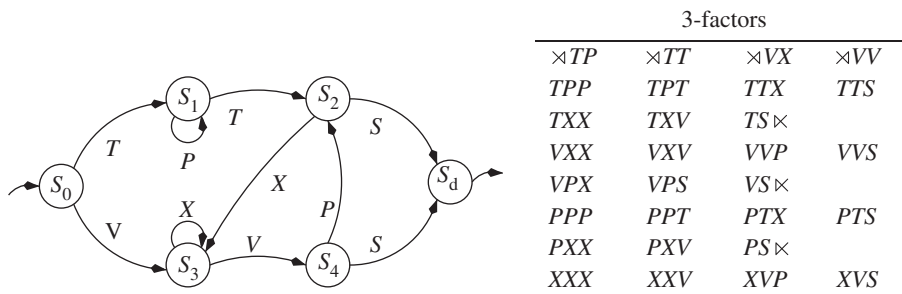
Figure 10. Reber's [30] grammar.
