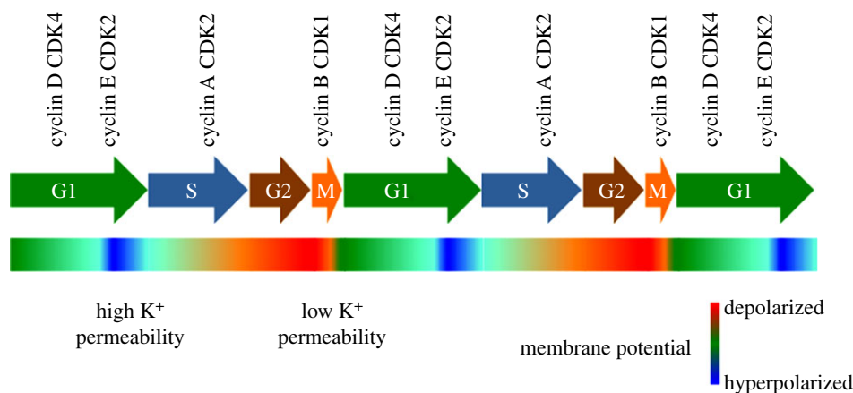
Figure 2. Schematic of the behaviour of the membrane potential along the cell cycle. Different potassium channels show variations of expression or activity through the cell cycle, thus shifting the membrane potential towards hyperpolarized values, close to the equilibrium potential for potassium, at the border between G1 and S-phases.
