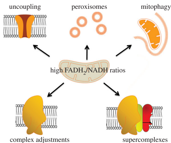
Figure 1. Schematic of possible adaptations to interior radical formation by respiratory chain complexes (especially complex I) upon catabolizing substrates with high FADH_2/NADH ratios. Clockwise: 1. Development of mechanisms to induce (regulated) mild uncoupling (e.g. uncoupling proteins). 2. Segregation of fatty acid oxidation (completely in neurons, plants and some yeasts, limited to VLCFAs only in most mammalian cells). 3. Evolving specific mitophagy pathways. Apart from mitophagy, a mitochondrion-associated decay (MAD) pathway appeared (resembling the ERAD pathway, see text). 4. Stimulating supercomplex formation, e.g. allowing complex I ‘direct’ access to its ‘own’ ubiquinone pool. 5. Adjusting complexes (especially I) and their synthesis to lessen both radical formation and its impact. Replacing complex I completely with Ndi1, as seen in Saccharomyces cerevisiae [30], can be seen as an extreme instance of the latter. (Online version in colour.)
